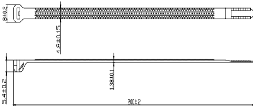
Drawing GC-200ST
